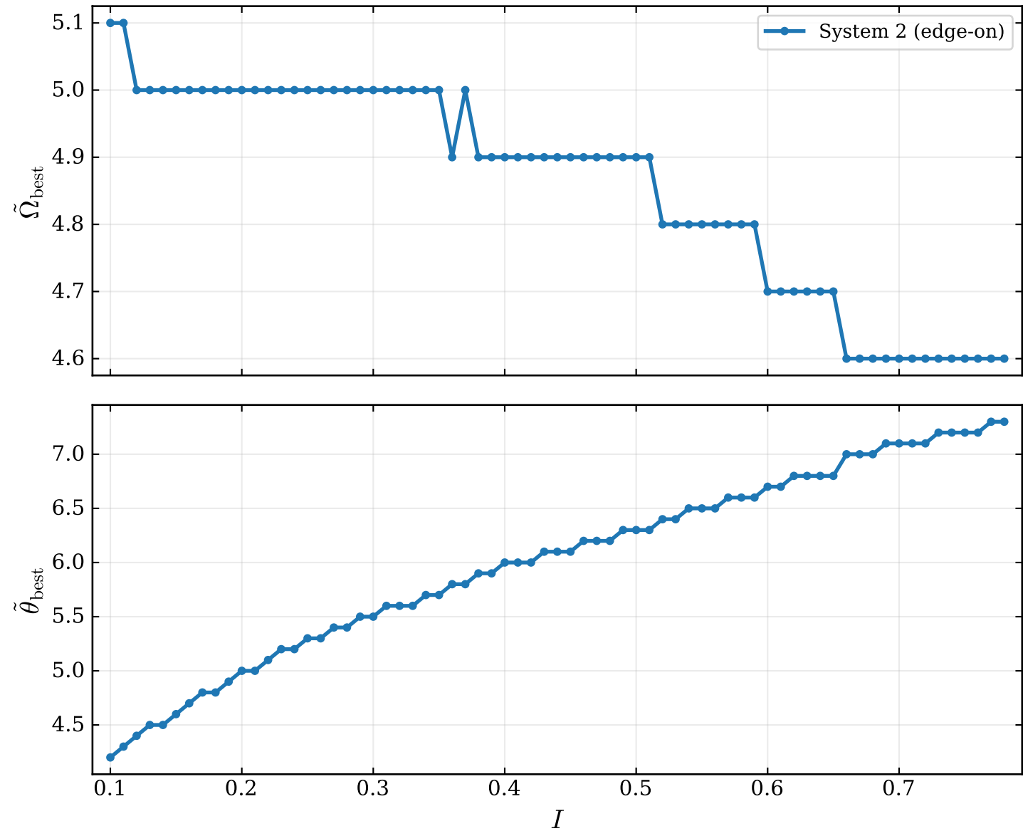
Best-matching precession parameters vs flux ratio ( \Delta t_d \approx 60 ms, z = 1 , \mathcal{M}_s = 15 M_\odot )
