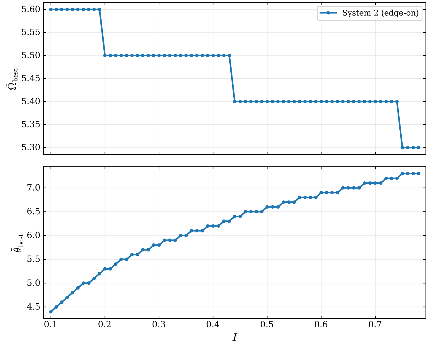
Best-matching precession parameters vs flux ratio ( \Delta t_{\text{d}} \approx 70 \text{ ms} , z = 1 , \mathcal{M}_{\text{s}} = 15 \text{ M}_{\odot} )
