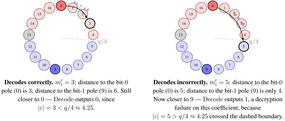
Figure 3.1: Decoding a true bit-0 coefficient on \mathbb{Z}_{17} . Red nodes decode to 0, blue nodes decode to 1, gray is the exact tie at 13; the bold red and blue nodes are Encode’s two poles, 0 and 9. Both panels start at the same pole and add noise \varepsilon — the only difference is whether \varepsilon stays under the dashed q/4 boundary (left) or crosses it (right).
