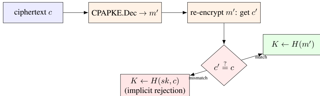
Figure 3.2: ML-KEM’s Decaps, schematically. The re-encryption check is the step the Fujisaki–Okamoto transform adds on top of plain Kyber.CPAPKE decryption; both branches must be computed in a way that reveals nothing about which one was taken.
