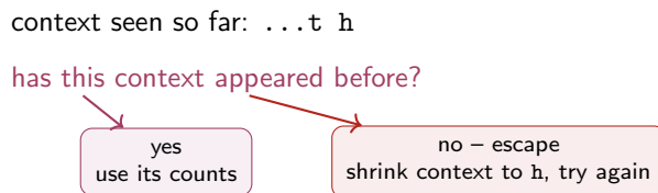
Figure 23: PPM’s escape mechanism. If the current context has statistics, PPM uses them directly (left, teal-magenta). If not, it shrinks the context by one symbol and tries again (right, red), repeating until it lands on a context it has actually seen.
