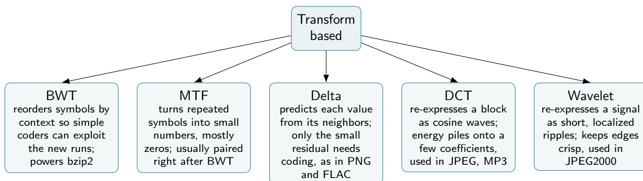
Figure 22: The five members of the transform-based family. Each reshapes data into a more compressible form and hands off to a downstream coder to do the actual squeezing – none of them saves a single bit on their own.
