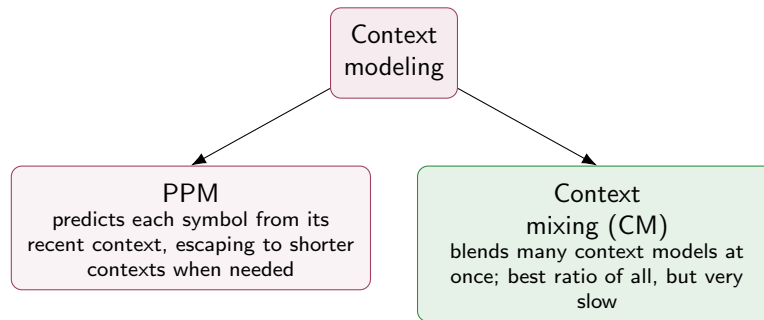
Figure 24: The context-modeling branch. Context mixing (green) sits at the extreme “best possible ratio” end of every trade-off curve we’ve drawn so far, paid for entirely in speed.
