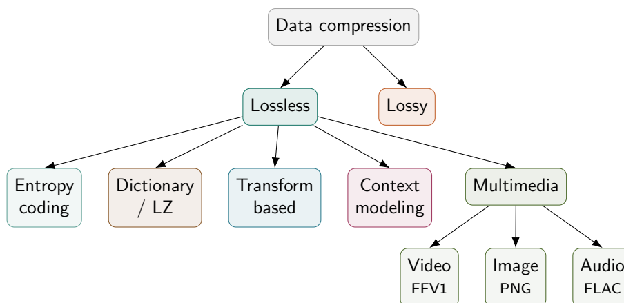
Figure 25: The master tree, stage 5: Lossless’s fifth child, Multimedia (olive) – the one we left empty back in figs. 5 and 15 – finally expands into the three media types we keep coming back to: video, image, and audio. Lossy is still collapsed on purpose; we expand it in Part 9 .
