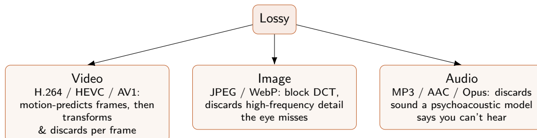
Figure 26: The lossy branch, fully grown. Video (left) builds directly on the same per-frame transform trick used for still images (middle), then adds motion prediction across frames. Audio (right) follows the same overall pattern – discard what perception can’t catch – using a hearing model instead of a vision model.
