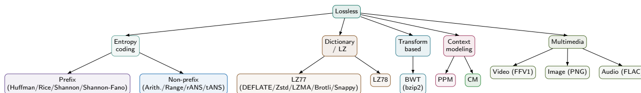
Figure 27: The complete tree, lossless half. Every colored leaf here is something we built up piece by piece over Parts 3 through 8.
