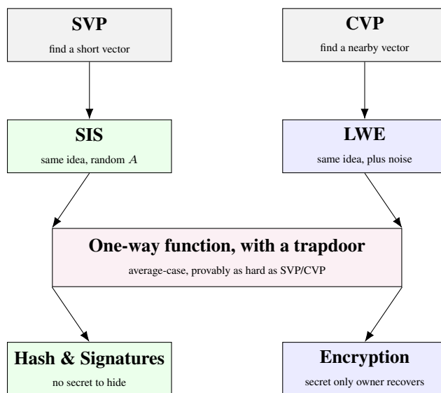
Figure 2.4: SIS and LWE are not a detour from SVP and CVP — they are SVP and CVP, restricted to a random, easy-to-sample family of lattices built from a matrix A . SIS lives on the kernel lattice \Lambda^\perp(A) (Section 2.4) and keeps SVP’s “find a short vector” shape; LWE lives on the image lattice \Lambda_q(A) (Section 2.5.5) and keeps CVP’s “find a nearby point” shape. That structural difference is exactly why the two problems power different cryptographic jobs: SIS’s kernel/short-vector shape gives you “no two things collide” (hash functions, signatures — nothing to hide), while LWE’s image/nearby-point shape gives you “there’s a hidden secret only the trapdoor-holder can recover” (encryption).
