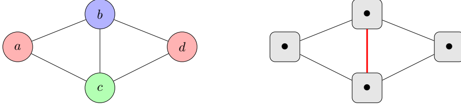
Graph with a proper 3-colouring \mathcal{C} ommitments; V picks edge bc and sees two different colours
