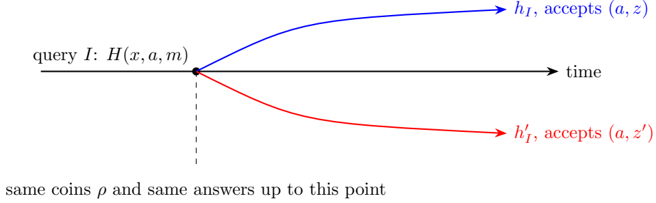
Figure 8.1: Forking: two executions diverge at the critical oracle query.
