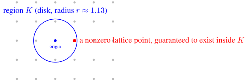
Figure 6: Minkowski’s First Theorem for L = \mathbb{Z}^2 ( \det(L) = 1 ): once the disk’s area exceeds 2^2 \cdot \det(L) = 4 (radius r \gtrsim 1.13 ), the theorem guarantees a nonzero lattice point lies inside it — and indeed (1, 0) (shown here relative to the chosen origin) is inside, at distance exactly 1 < 1.13 .
