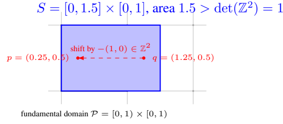
Figure 5: Blichfeldt's Lemma in action for L = \mathbb{Z}^2 . S (blue) has area 1.5, exceeding \det(L) = 1 , so it cannot fit inside one fundamental domain without “spilling over.” The spillover — the sliver of S with x \in [1, 1.5] — folds back (shift by -(1, 0) ) into the same unit square as the rest of S , and lands on top of it: the two marked points p, q \in S fold to the same location, and p - q = (-1, 0) is a nonzero lattice vector, exactly as the lemma guarantees.
