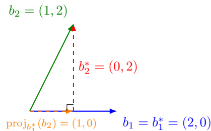
Figure 2: The geometry behind one Gram–Schmidt step (numbers match the worked example below). The green vector b_2 decomposes into an orange piece — its projection onto b_1^* , i.e. “how much of b_2 points along b_1^* ” — and a red perpendicular leftover, b_2^* = b_2 - \text{proj}_{b_1^*}(b_2) . That red leftover, translated back to the origin, is the new orthogonal basis vector. Every step of Gram–Schmidt is this same picture, repeated once per previous direction.
