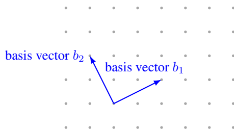
Figure 4: A 2-dimensional, full-rank lattice generated by a basis \{b_1, b_2\} : every grid dot is reachable by some integer combination a_1b_1 + a_2b_2 (with a_1, a_2 \in \mathbb{Z} ), starting from any chosen origin dot. This is the same object as the subgroup definition above — just viewed through its basis instead of as an abstract subgroup.
