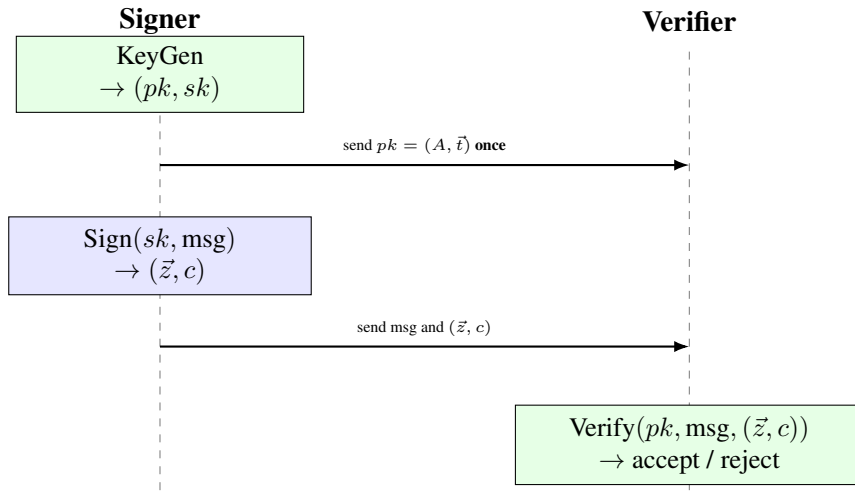
Figure 4.1: The ML-DSA protocol, party by party. Unlike ML-KEM’s exchange (Figure 3.1), where both parties run one algorithm each per session, here only the Signer ever runs KeyGen and Sign — the secret key sk = (\vec{s}_1, \vec{s}_2) never leaves the Signer. pk = (A, \vec{t}) is generated and published once (e.g. embedded in a certificate) and then reused for every subsequent message; each new msg only needs a fresh (\vec{z}, c) pair traveling alongside it. The Verifier never runs KeyGen or Sign at all — Verify is the Verifier’s only algorithm, and it can be run by anyone holding pk , independently, with no reply sent back to the Signer.
