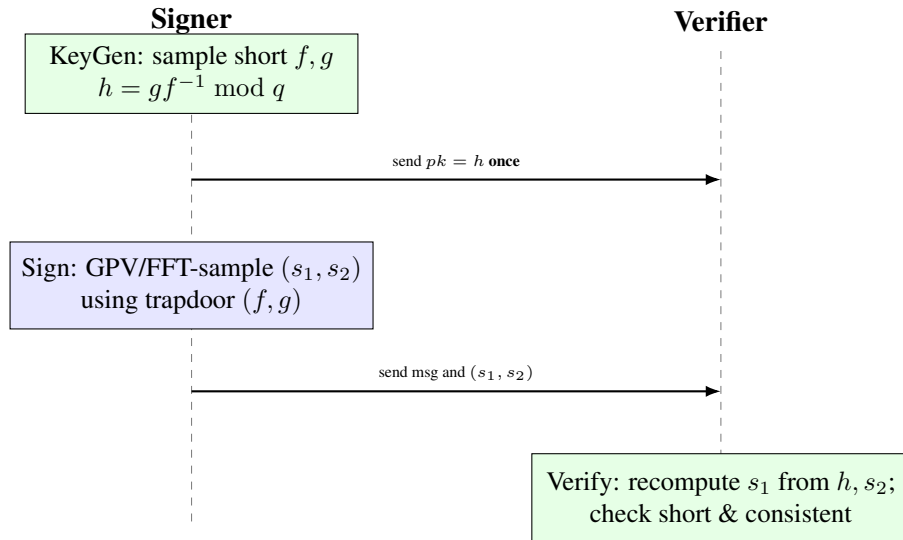
Figure 4.2: FN-DSA’s protocol shape, side by side with Figure 4.1: identical party structure to ML-DSA — only the Signer ever touches the trapdoor (f, g) , and only the Signer runs KeyGen and Sign; the Verifier holds nothing but the public h and runs Verify alone, with no reply sent back. What changes is entirely internal to the Signer’s Sign step: instead of Dilithium’s commit/challenge/response loop with rejection sampling, Falcon runs a single GPV trapdoor-guided sampling step (fast Fourier sampling) directly against the hashed message target — the external protocol shape is the same, but there is no “discard and retry” loop here the way there is in Dilithium’s Sign (Algorithm 2).
