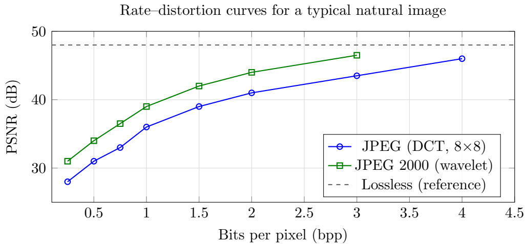
Figure 9: Typical rate-distortion curves. At any given bit-rate, JPEG 2000 (wavelet) outperforms JPEG, but JPEG remains competitive for \text{bpp} > 1 .
