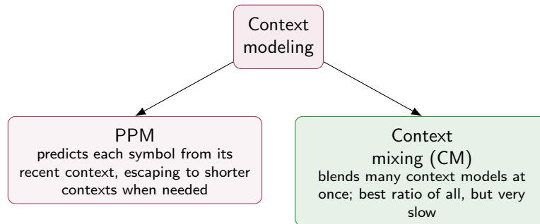
Figure 24: The context-modeling branch. Context mixing (green) sits at the extreme “best possible ratio” end of every trade-off curve we’ve drawn so far, paid for entirely in speed.
