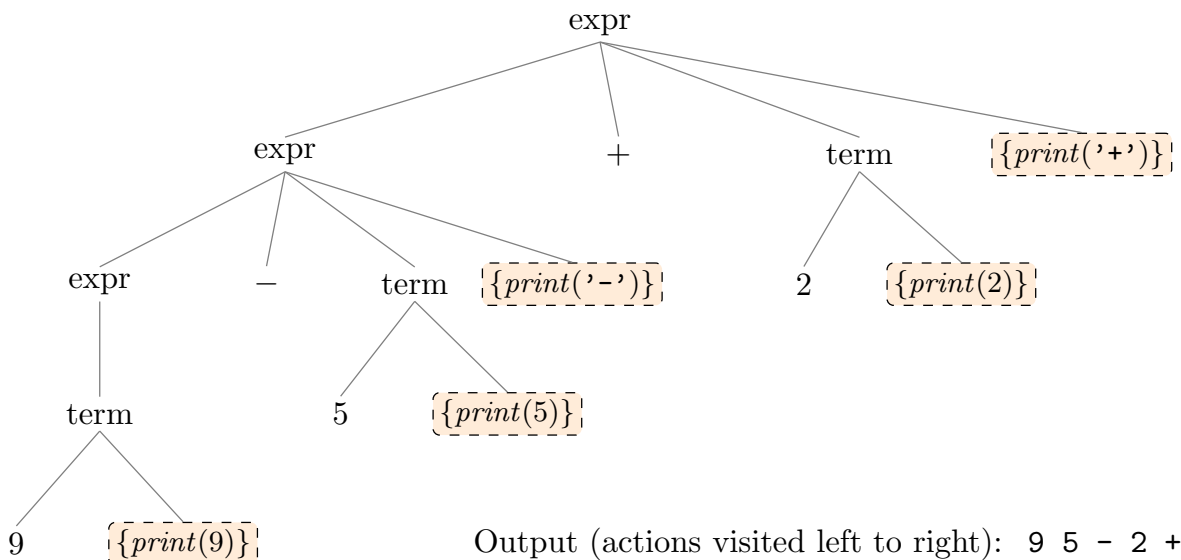
Figure 5: Parse tree of 9-5+2 with actions (dashed boxes) as extra children. Visiting the tree depth-first, left to right, executes the actions in the order 9, 5, -, 2, +, producing the postfix form.
