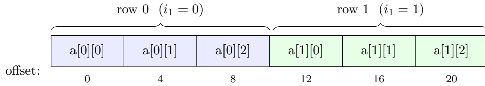
Figure 6: Row-major layout of int a[2][3] ( w = 4 ). Offset of a[i][j] is i \times 12 + j \times 4 .
