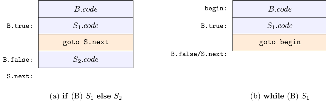
Figure 7: Layout of the generated code. B.code contains jumps to B.true or B.false ; it “falls through” to neither, so the labels can be placed anywhere.
