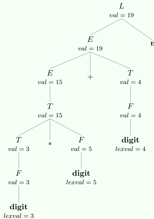
Figure 3: Annotated parse tree for 3*5+4 \mathbf{n} . Each node shows the value of its synthesized attribute val .
