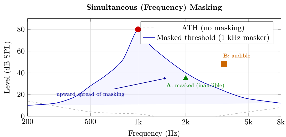
Figure 13: Simultaneous (frequency) masking. A loud 1 kHz masker at 80 dB SPL raises the hearing threshold over a wide frequency range (blue curve). Maskee A at 2 kHz and 35 dB falls below the masked threshold — it is completely inaudible despite being above the ATH. Maskee B at 3.5 kHz and 48 dB is above the masked threshold and therefore audible. Notice the asymmetry: masking spreads more strongly upward (to higher frequencies) than downward.
