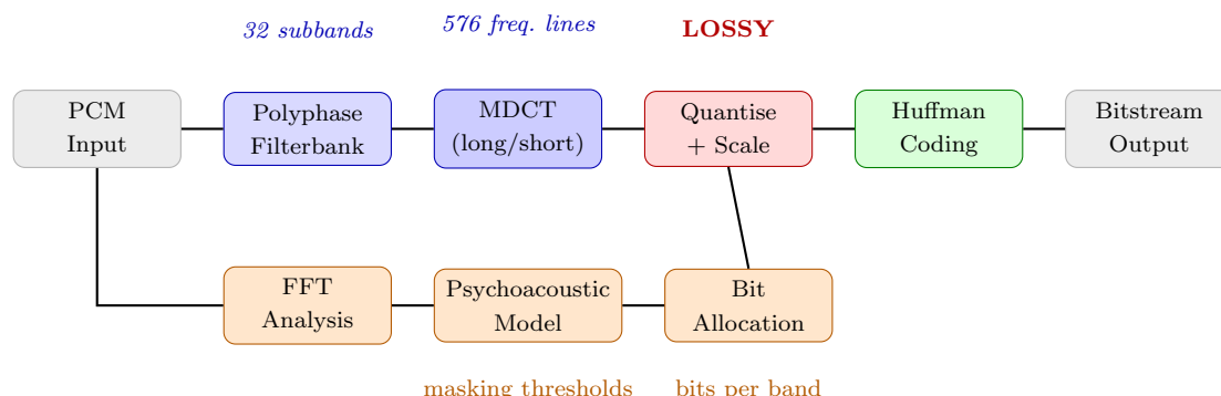
Figure 16: Complete MP3 encoding pipeline. The top path is the main audio processing chain. The bottom path is the psychoacoustic model, which runs in parallel (using an FFT for high-resolution spectral analysis) and feeds the bit allocation module. Only the quantisation stage is irreversible.
