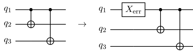
Figure 13: A single error on the first gate in the encoding circuit propagates to affect all subsequent qubits. This “error spreading” is the key danger that fault-tolerant design must prevent.
