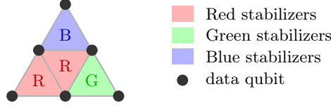
Figure 17: A small portion of a 2D color code lattice. Each colored face contributes both an X -type and a Z -type stabilizer on its vertices. The 3-colorability allows fault-tolerant gates beyond those of the surface code.
