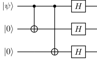
Figure 6: Phase-flip code encoding: first encode with CNOTs (as in the bit-flip code), then apply Hadamard to each qubit.
