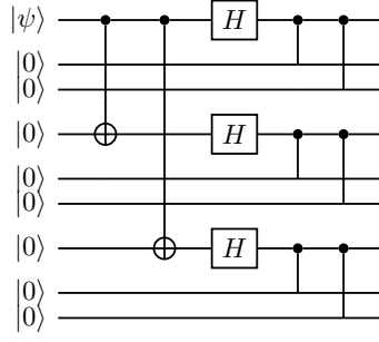
Figure 8: Shor code encoding circuit (simplified). First two CNOTs copy the logical qubit to qubits 4 and 7 (phase-flip structure). Then Hadamards create superpositions. Finally CNOTs within each block of three create the bit-flip structure. Rows 2–3, 5–6, 8–9 receive the CNOT targets from their respective block leaders.
