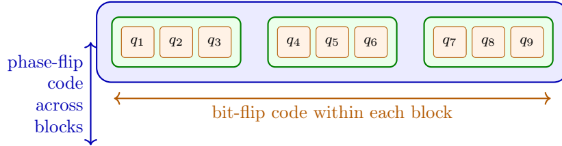
Figure 7: The nested structure of the Shor 9-qubit code. Three groups of three qubits each form a bit-flip code. Across the three groups, the overall structure forms a phase-flip code.
