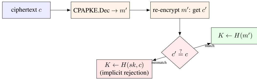
Figure 3.1: ML-KEM’s Decaps, schematically. The re-encryption check ( c' \stackrel{?}{=} c ) is the step the Fujisaki–Okamoto transform adds on top of plain Kyber.CPAPKE decryption — and, because both branches must be computed in a way that reveals nothing about which branch was taken (equal time, no data-dependent memory access), it is also one of the most scrutinized few lines of code in the entire scheme from a side-channel perspective.
