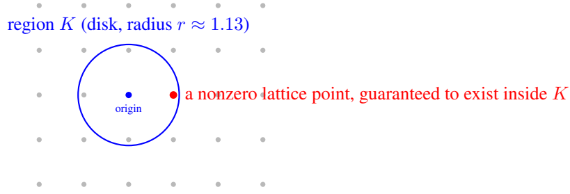
Figure 5: Minkowski’s First Theorem for L = \mathbb{Z}^2 ( \det(L) = 1 ): once the disk’s area exceeds 2^2 \cdot \det(L) = 4 (radius r \gtrsim 1.13 ), the theorem guarantees a nonzero lattice point lies inside it — and indeed (1, 0) (shown here relative to the chosen origin) is inside, at distance exactly 1 < 1.13 .
