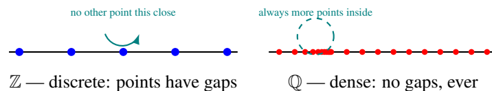
Figure 3: Discreteness, visualized. Left: in \mathbb{Z} , every point has a gap of size 1 around it with nothing else nearby — discrete. Right: in \mathbb{Q} , no matter how small a circle you draw around a point, there are always infinitely many more rational points crammed inside it — dense, and therefore not discrete.
