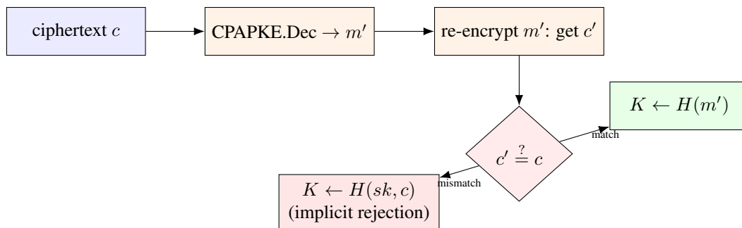
Figure 3.1: ML-KEM’s Decaps, schematically. The re-encryption check ( c' \stackrel{?}{=} c ) is the step the Fujisaki–Okamoto transform adds on top of plain Kyber.CPAPKE decryption — and, because both branches must be computed in a way that reveals nothing about which branch was taken (equal time, no data-dependent memory access), it is also one of the most scrutinized few lines of code in the entire scheme from a side-channel perspective.
