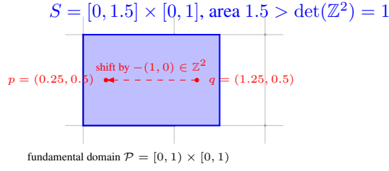
Figure 6: Blichfeldt's Lemma in action for L = \mathbb{Z}^2 . S (blue) has area 1.5, exceeding \det(L) = 1 , so it cannot fit inside one fundamental domain without “spilling over.” The spillover — the sliver of S with x \in [1, 1.5] — folds back (shift by -(1, 0) ) into the same unit square as the rest of S , and lands on top of it: the two marked points p, q \in S fold to the same location, and p - q = (-1, 0) is a nonzero lattice vector, exactly as the lemma guarantees.
