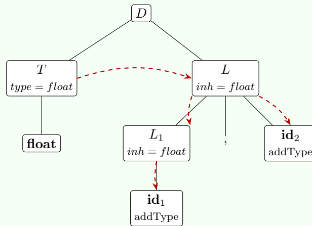
Figure 6: Parse tree for float id 1 , id 2 with dependency edges (dashed) for the inherited attribute inh .
