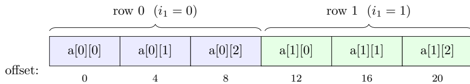
Figure 8: Row-major layout of int a[2][3] ( w = 4 ). Offset of a[i][j] is i \times 12 + j \times 4 .
