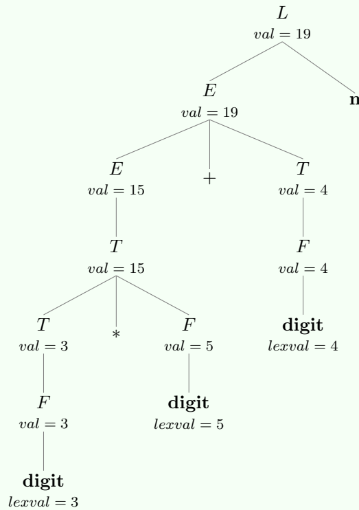
Figure 5: Annotated parse tree for 3*5+4 n . Each node shows the value of its synthesized attribute val .
