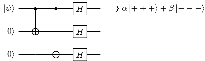
Figure 7: Phase-flip code encoding. CNOTs spread the information across three qubits (as in the bit-flip code); Hadamard gates then rotate each qubit from the Z basis into the X basis.
