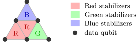
Figure 21: A small portion of a 2D color code lattice. Each colored face contributes both an X -type and a Z -type stabilizer on its vertices. The 3-colorability allows fault-tolerant gates beyond those of the surface code.
