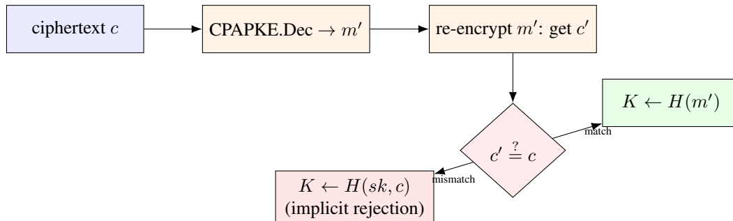
Figure 3.1: ML-KEM’s Decaps, schematically. The re-encryption check is the step the Fujisaki–Okamoto transform adds on top of plain Kyber.CPAPKE decryption; both branches must be computed in a way that reveals nothing about which one was taken.
