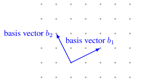
Figure 1.4: A 2-dimensional, full-rank lattice generated by a basis \{b_1, b_2\} : every grid dot is reachable by some integer combination a_1b_1 + a_2b_2 (with a_1, a_2 \in \mathbb{Z} ), starting from any chosen origin dot. This is the same object as the subgroup definition above — just viewed through its basis instead of as an abstract subgroup.
