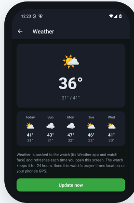
Companion → Weather
