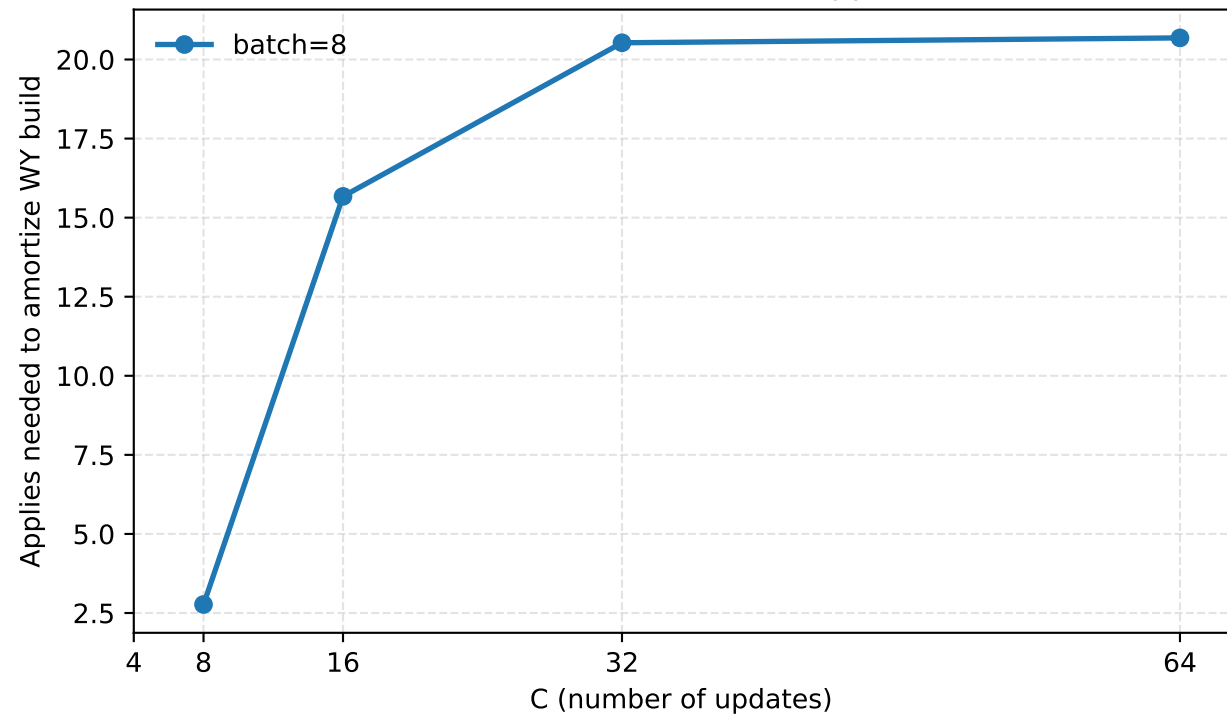
Break-even Number of Applies
