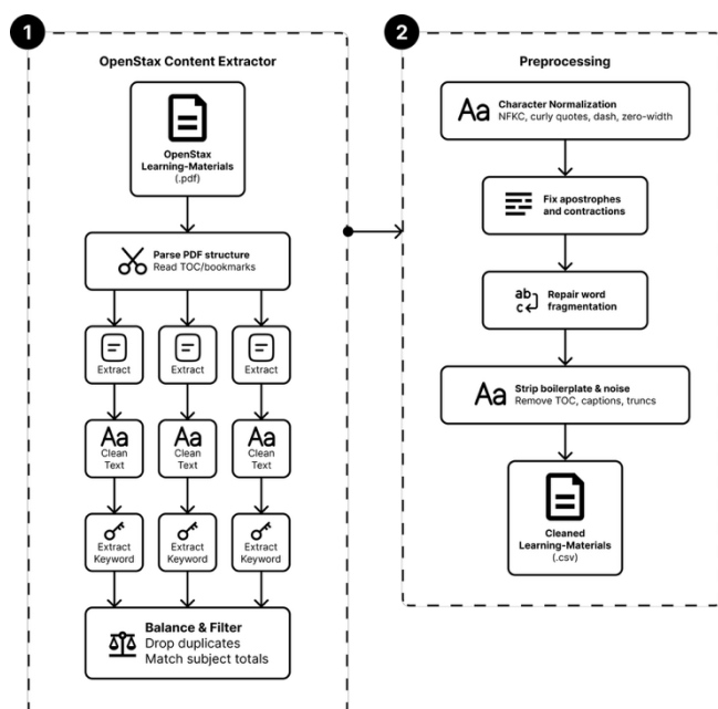
Fig. 2. OpenStax two-stage preprocessing pipeline. removed.
