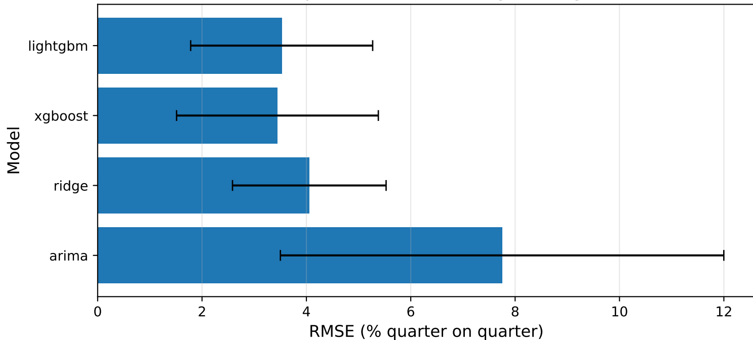
Model comparison: RMSE on regime-aligned CV
