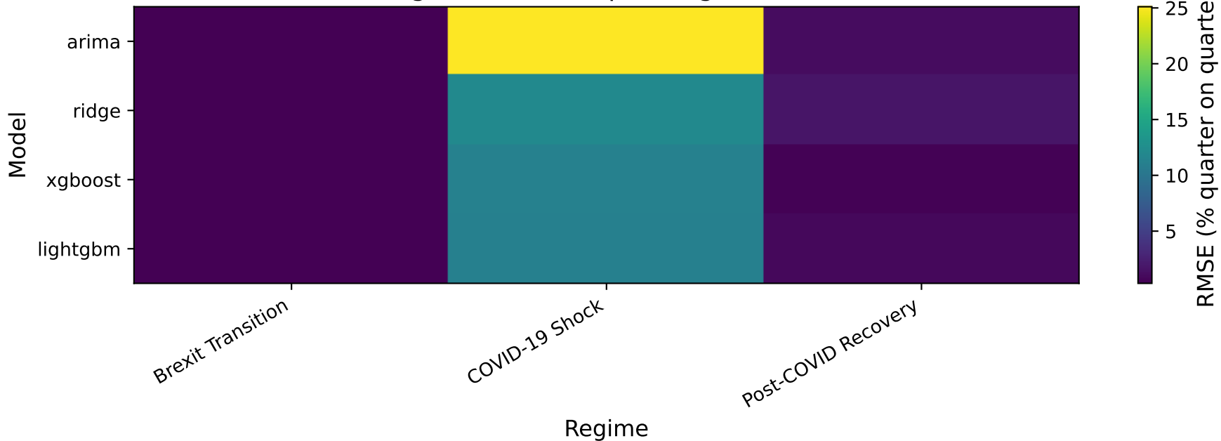
Per-regime RMSE (expanding-window CV)
