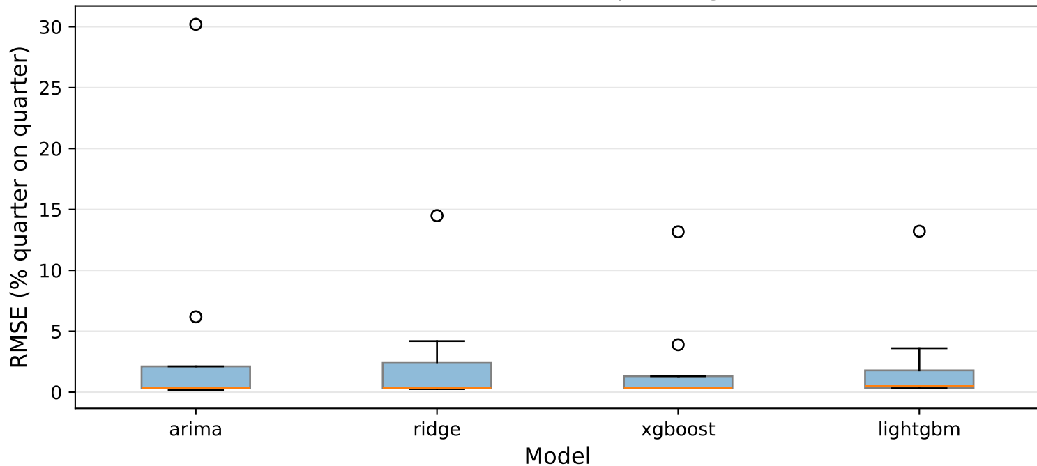
Per-fold RMSE distribution (expanding-window CV)
