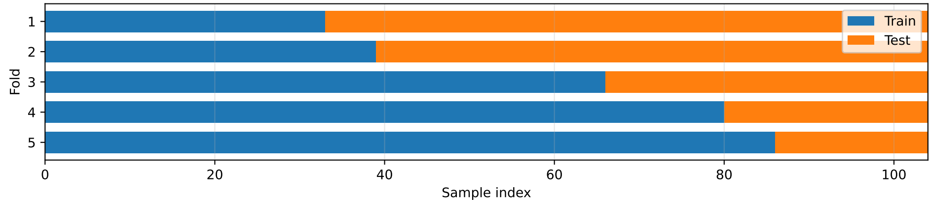
Regime-aligned CV
