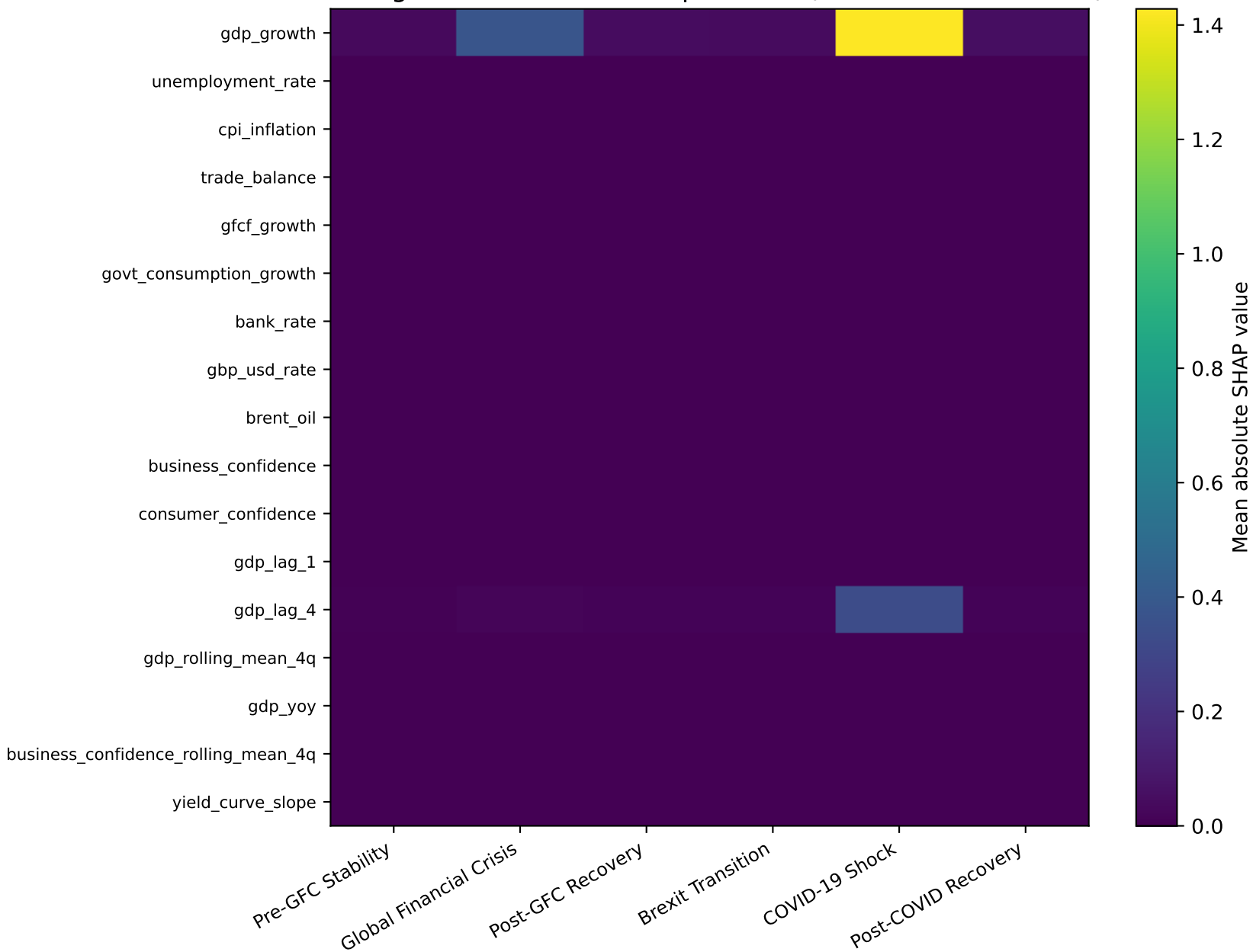
Per-regime SHAP feature importance (mean absolute SHAP)
