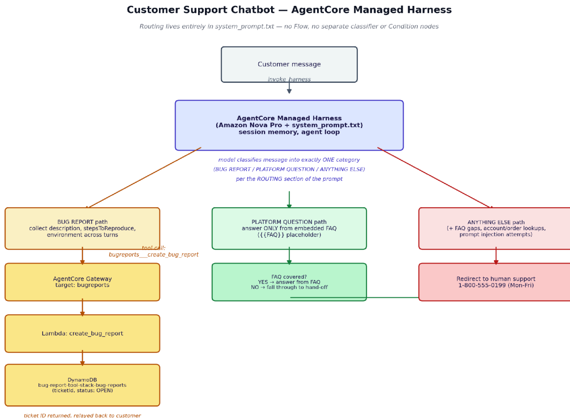
Figure 1. Customer messages flow through the AgentCore harness, showing all three routing paths and the bug-report tool chain (Gateway → Lambda → DynamoDB).
