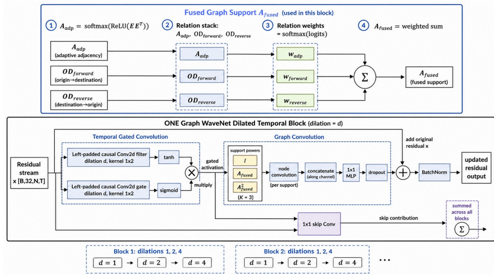
图 4-4 Graph WaveNet 时空块与支撑图细节
