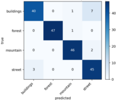
Task 4 — Confusion matrix (validation)
