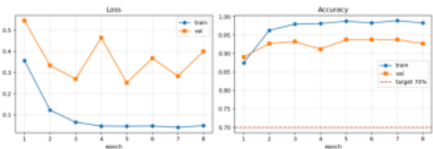
Task 4 — Training / validation curves
