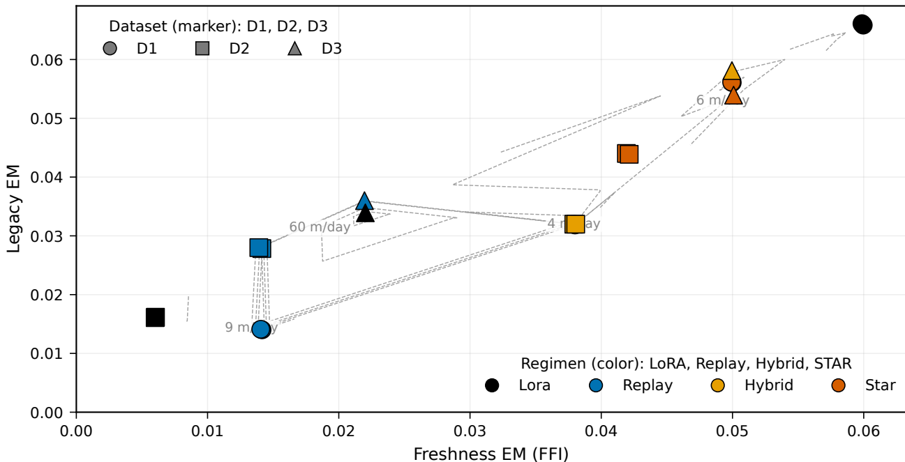
Pareto frontier with iso-cost overlays (TinyLlama, D1-D3)
