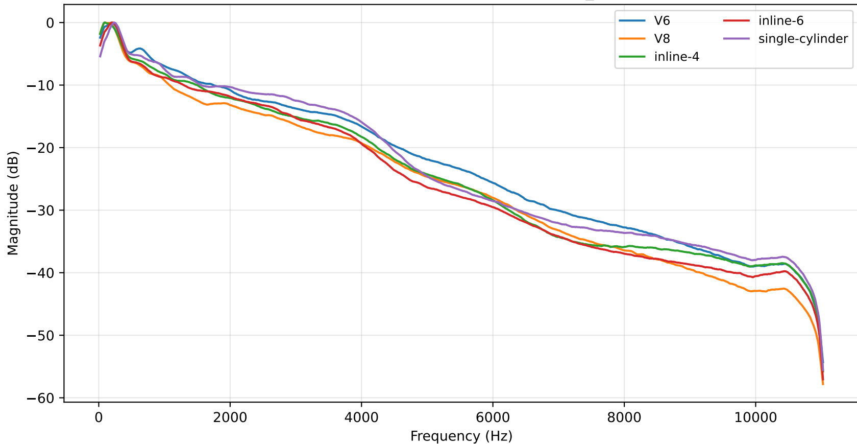
Overlay: Mean Spectrum per Class — engine_configuration
