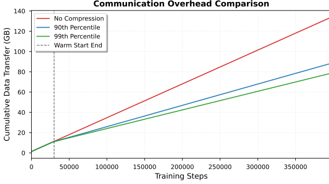
Fig. 2. Cumulative network transfer comparison. Gradient accumulation with 90th percentile threshold reduces data transfer by 34%, saving 45.48 GB over 400,000 training steps.
