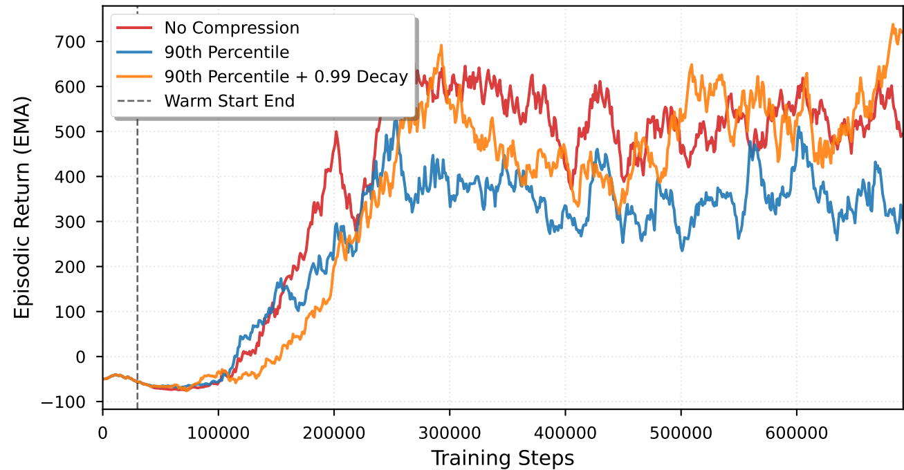
Training Performance Comparison (Concurrent Runs)
