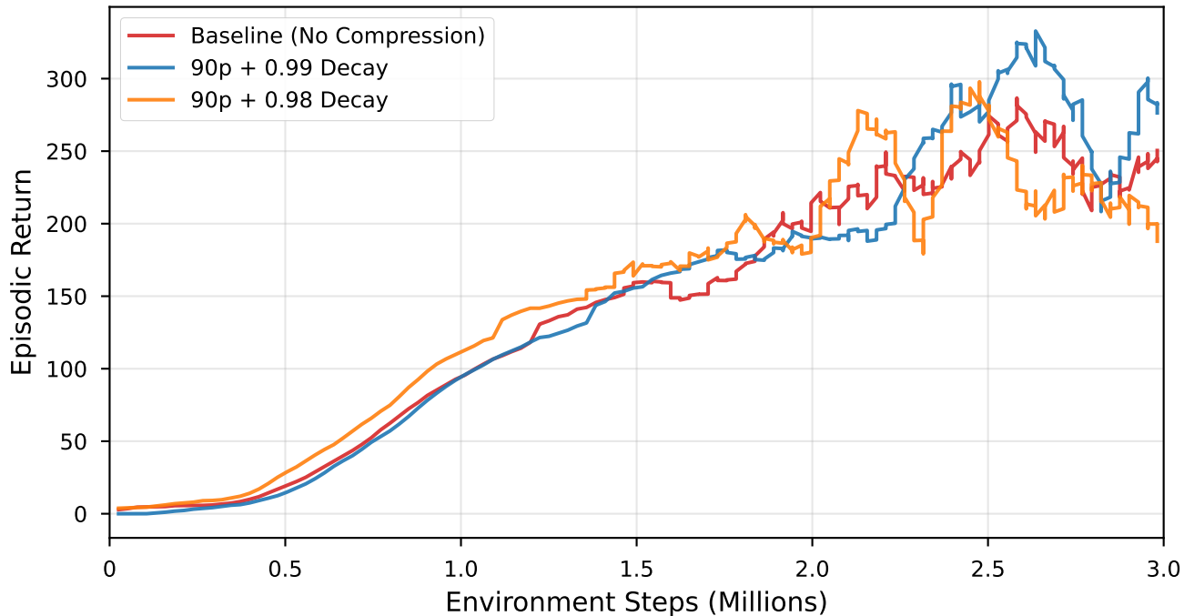
Enduro — Gradient Compression vs Baseline
