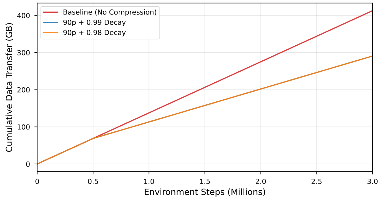
Enduro — Cumulative Data Transfer
