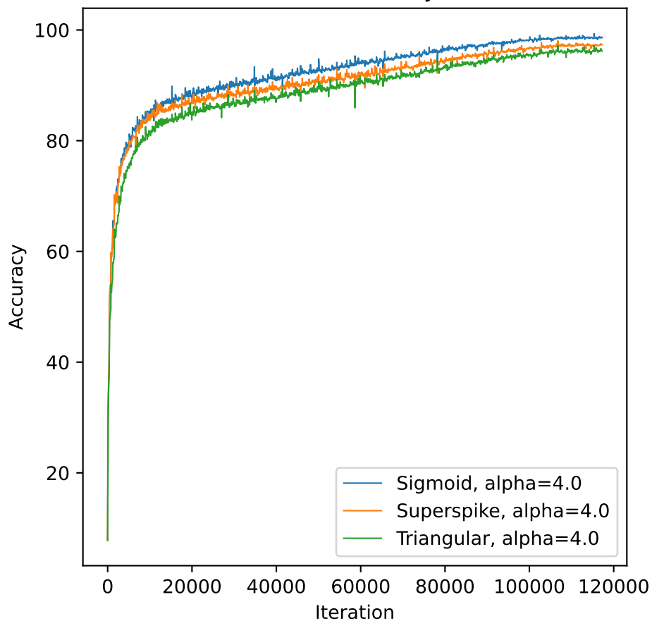
Validation Accuracy
