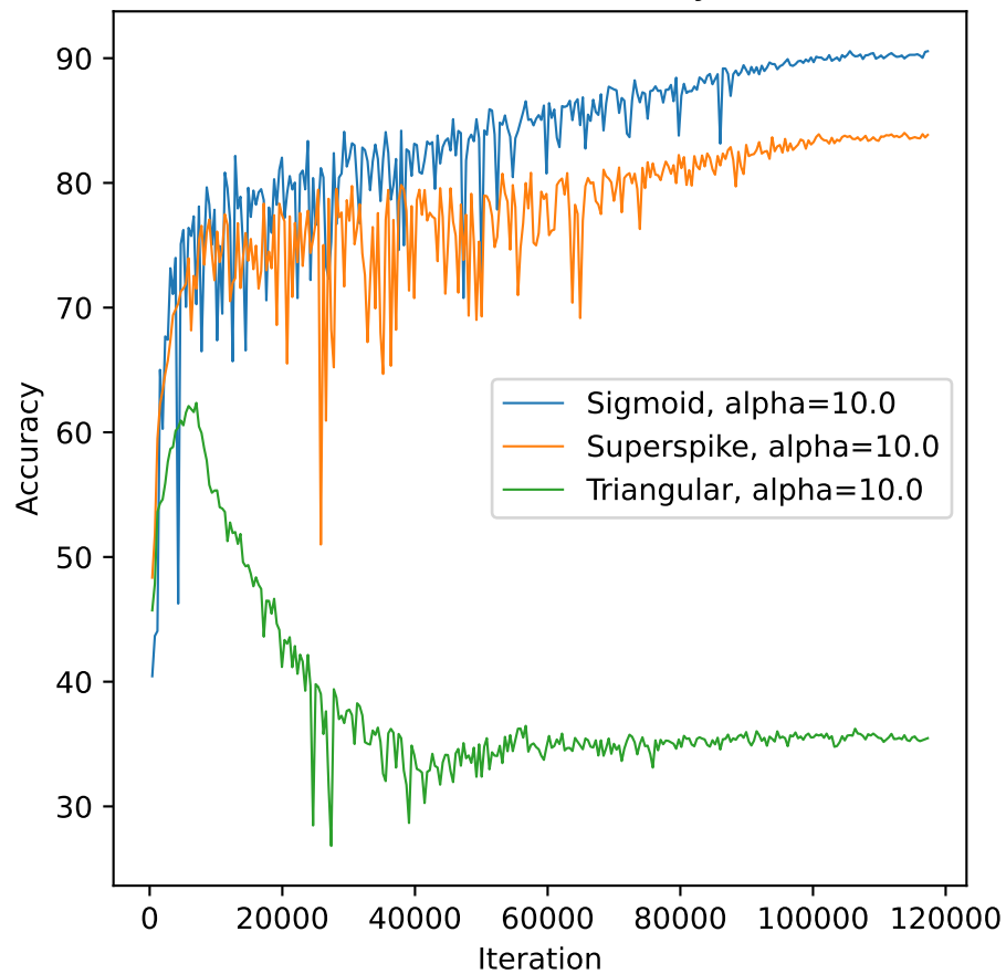
Validation Accuracy
