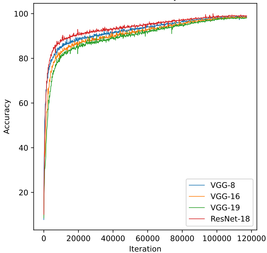
Validation Accuracy
