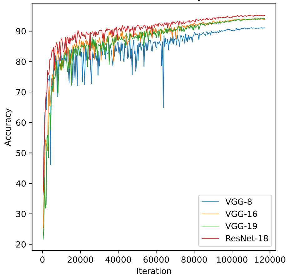
Validation Accuracy
