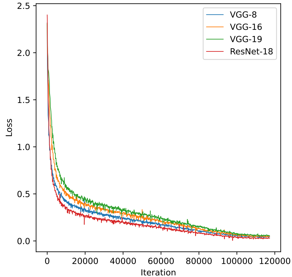
Validation Loss
