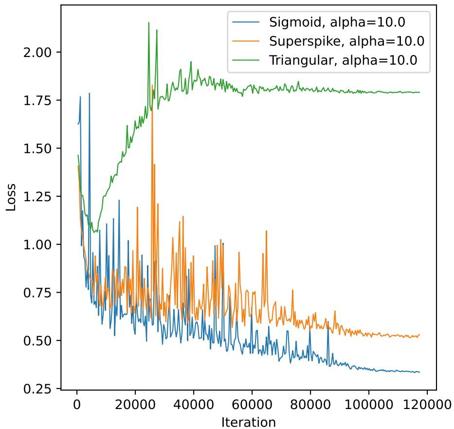
Validation Loss
