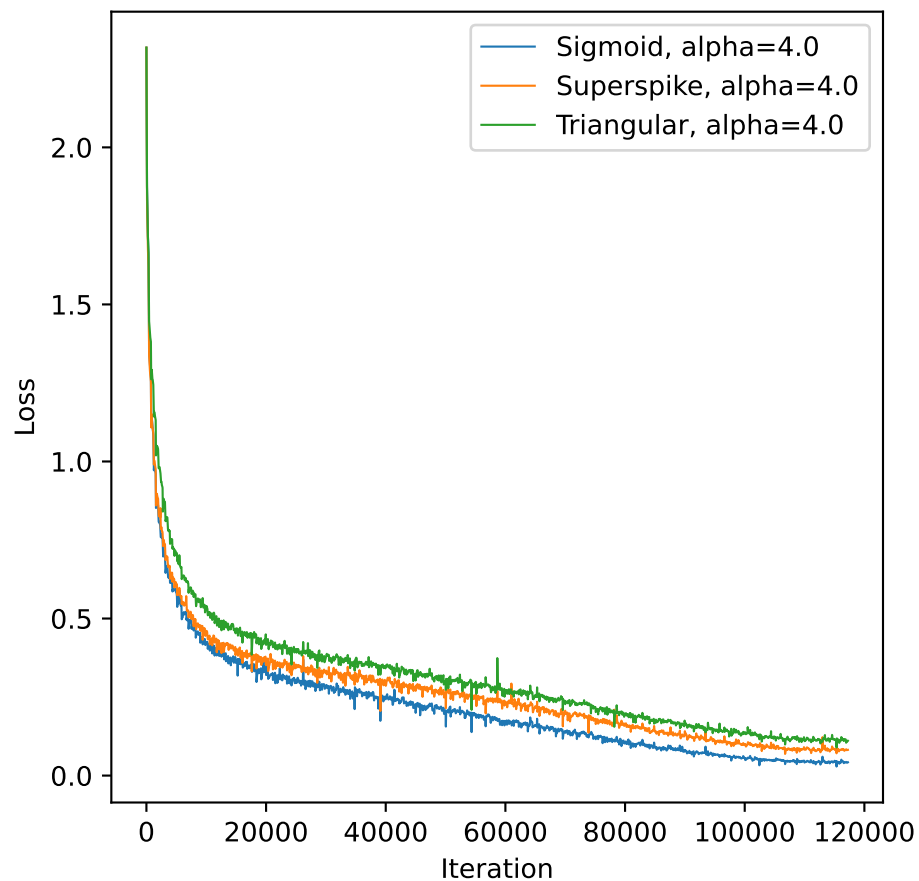
Validation Loss
