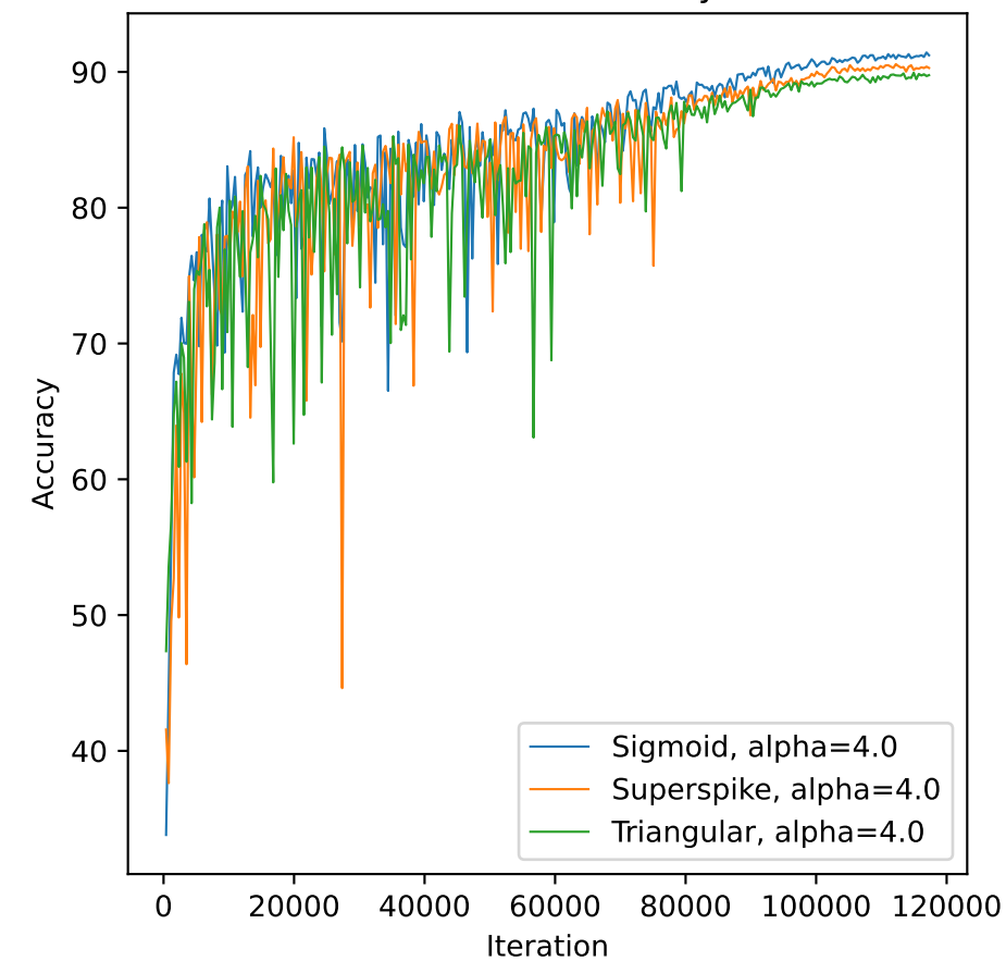
Validation Accuracy
