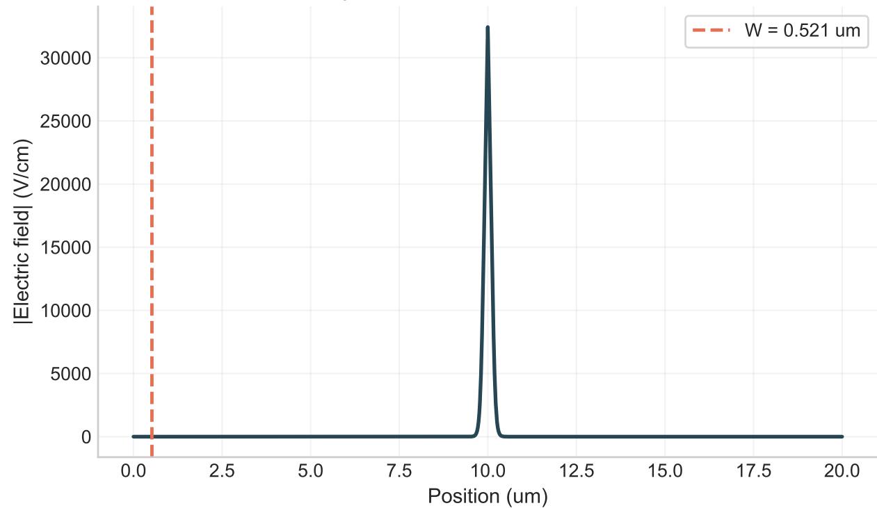
Equilibrium Electric Field Profile
