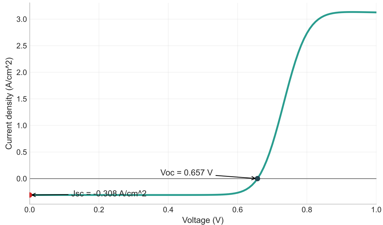
Illuminated J-V with J_{sc} and V_{oc}
