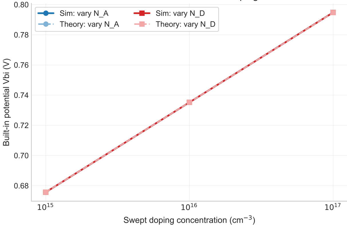
Built-in Potential versus Doping
