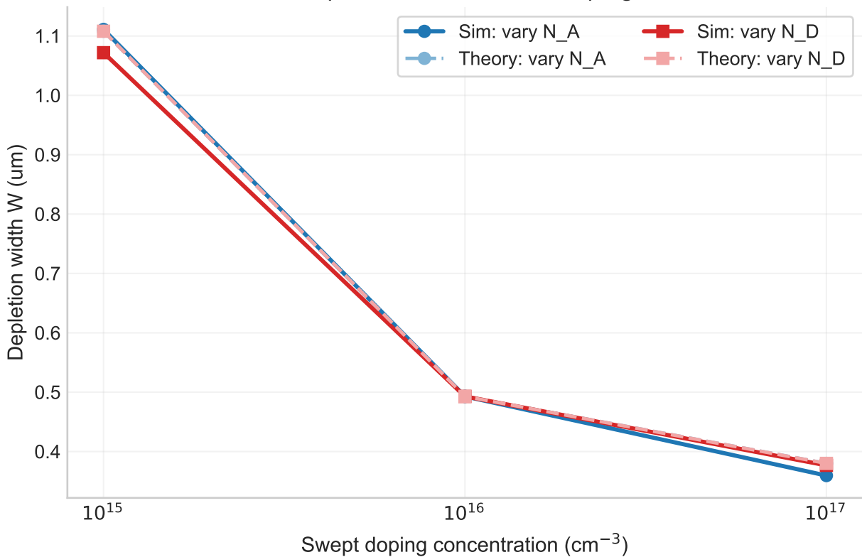
Depletion Width versus Doping
