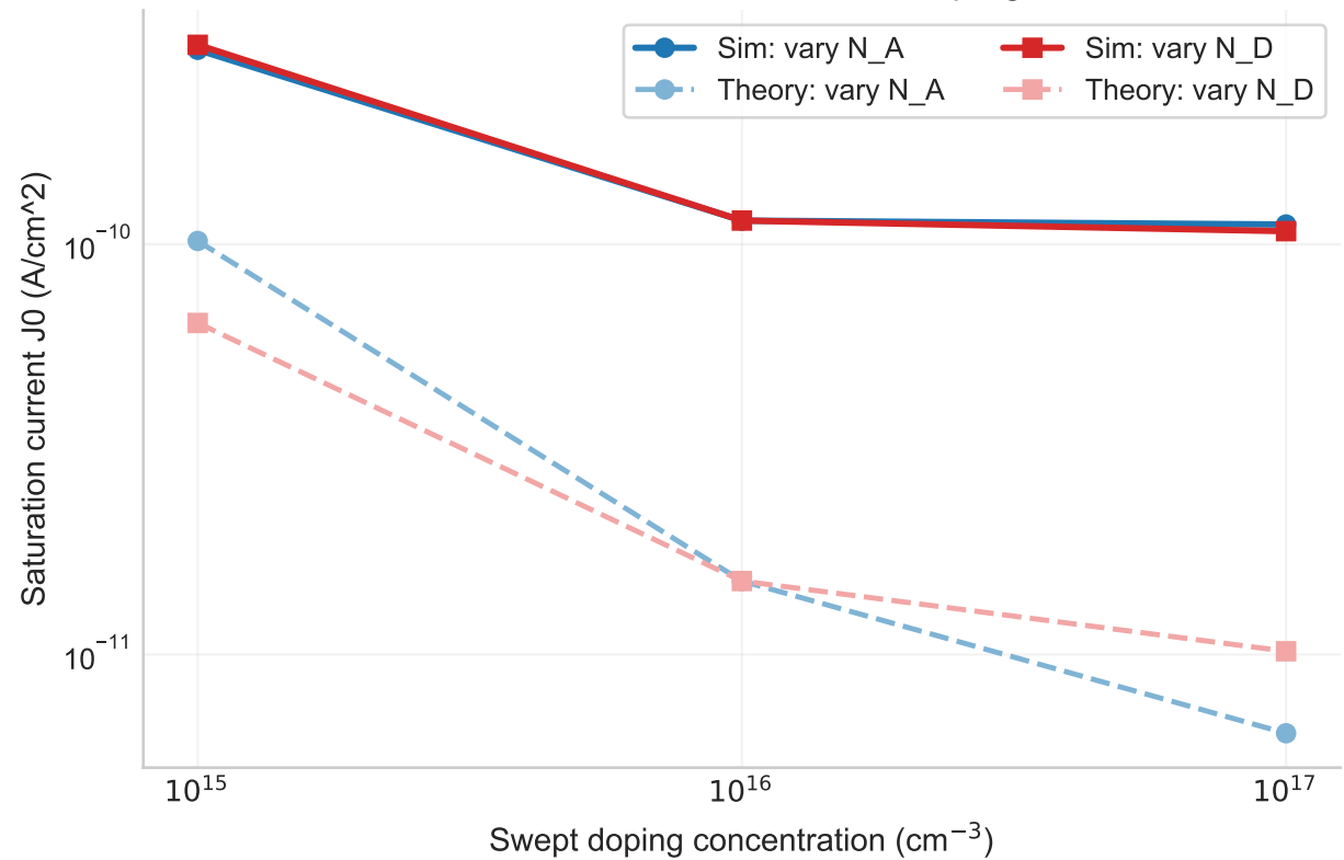
Saturation Current versus Doping
