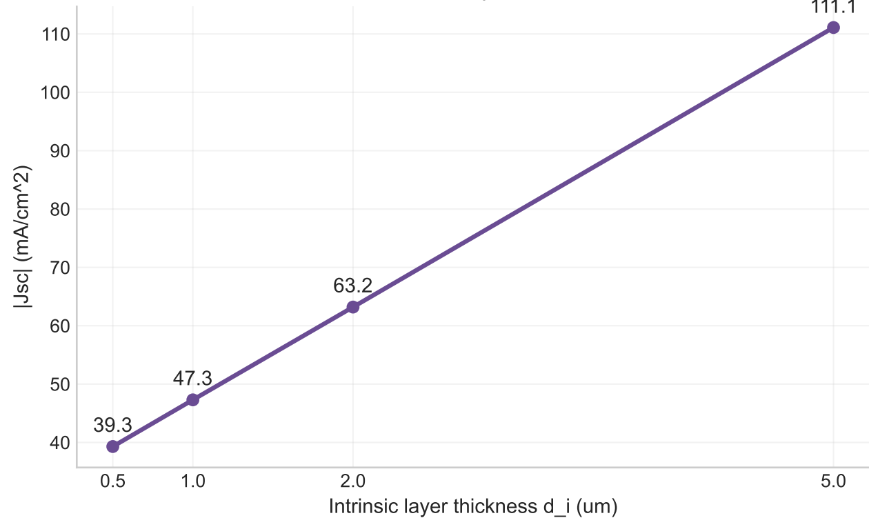
PIN Thickness Dependence of J_{sc}
