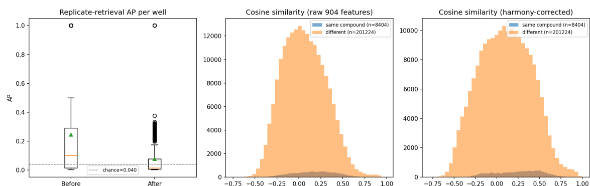
Replicate retrieval AP and similarity distributions
