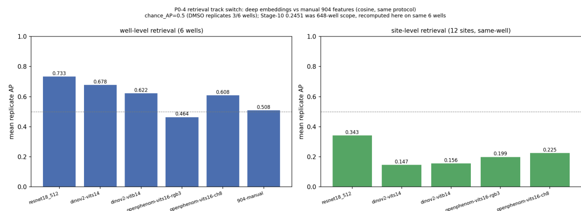
Retrieval track switch
