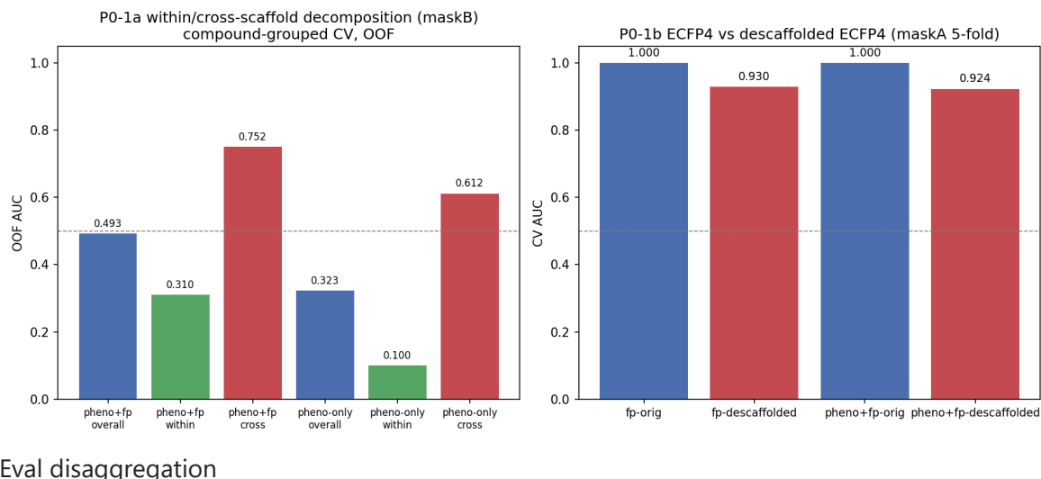
Figure 29a: within- vs cross-scaffold CV decomposition (P0-1a) underlying the protocol decision in §24.2.
