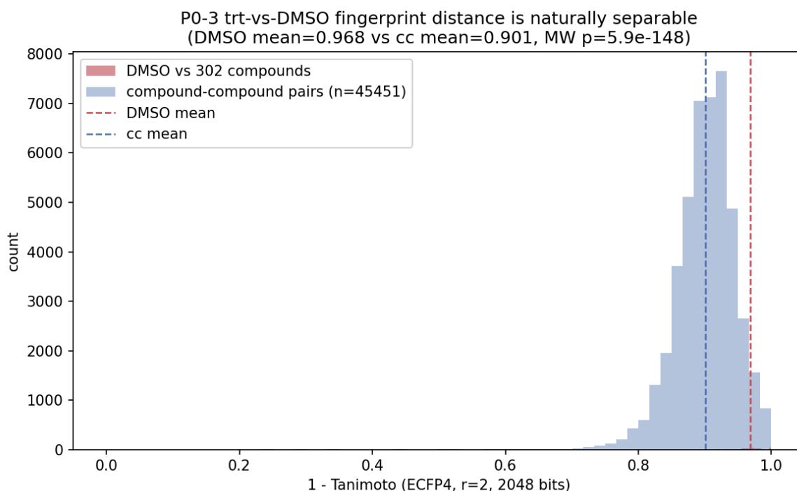
FP distance distribution
