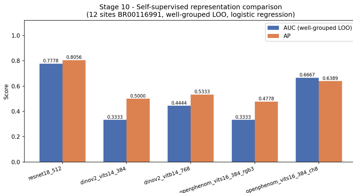
Self-supervised representation comparison
