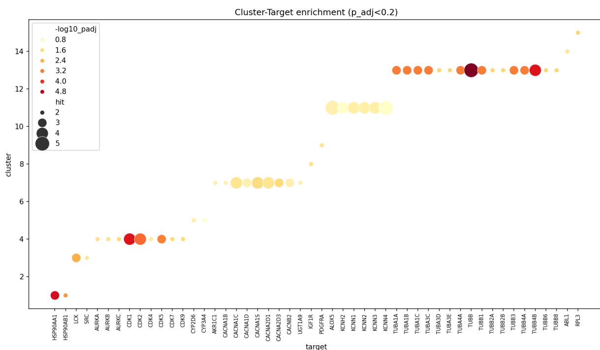
Target enrichment
