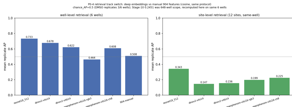
Retrieval track switch
