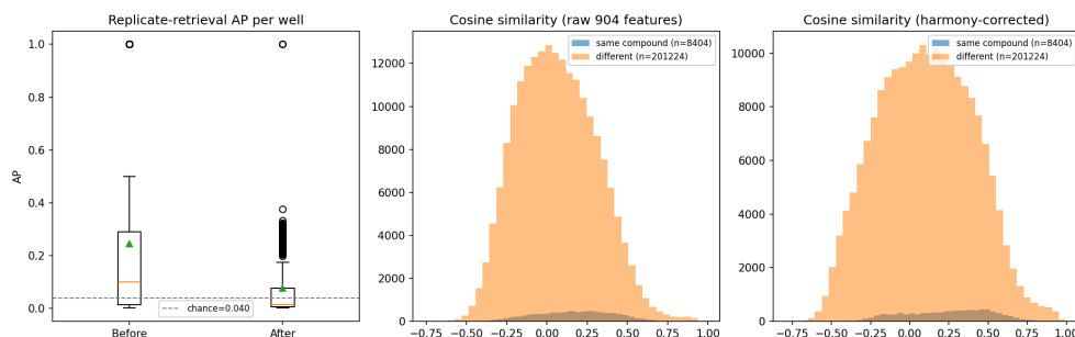
Replicate retrieval AP and similarity distributions
